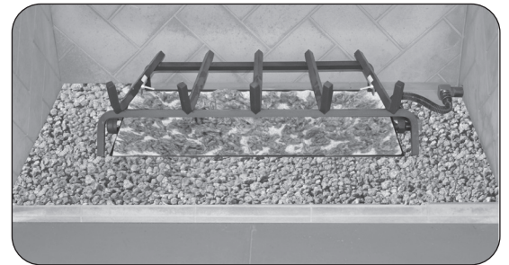
Fig. 13-3 Place grate
