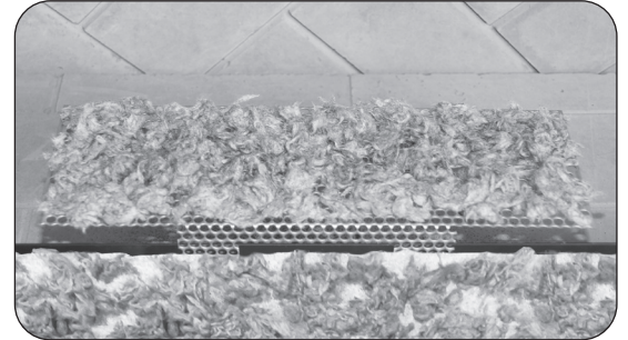
Fig. 13-2 Cover screen with embers
