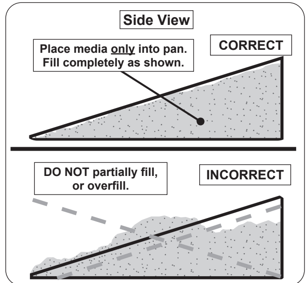
Fig. 12-2 Correct/Incorrect media placement (sand or vermiculite)
