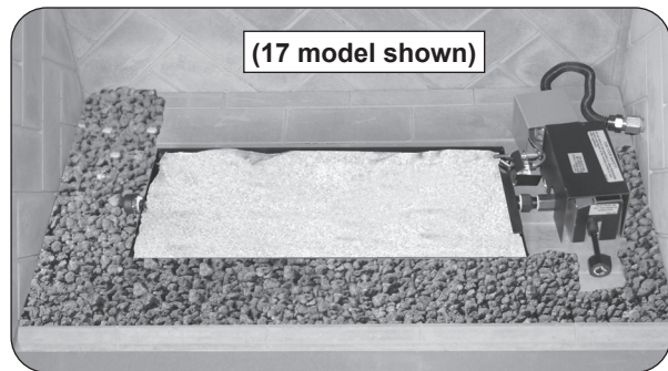
Fig. 19-1 Place sand/vermiculite
