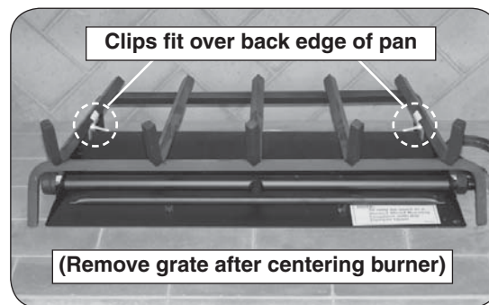
Fig. 10-2 Position grate
