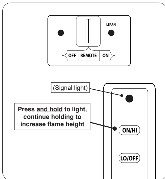
Fig. 35-1 Remote lighting
