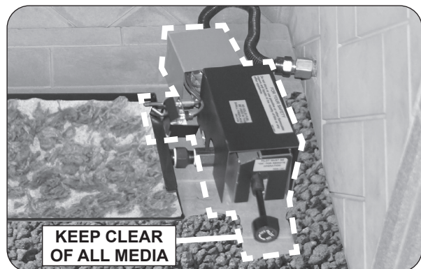
Fig. 19-4 Keep pilot, valve, & shield(s) clear
