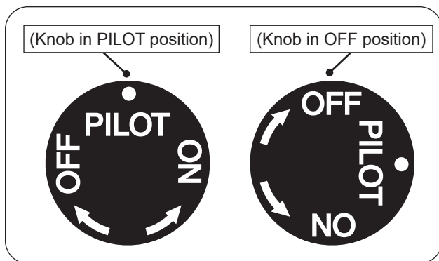
Fig. 24-2 Manual shut down
