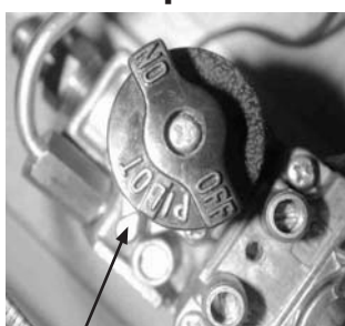
Fig. 29-2 PILOT position
