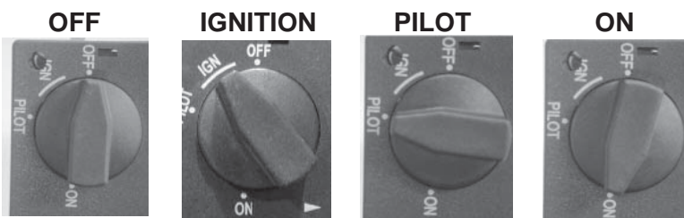
Gas valve operating positions Fig. 27-1
