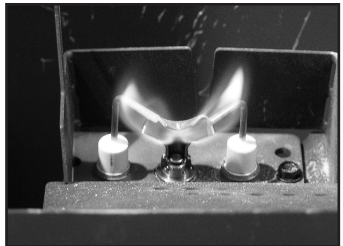
Figure 4.1 IPI Pilot Flame Patterns
