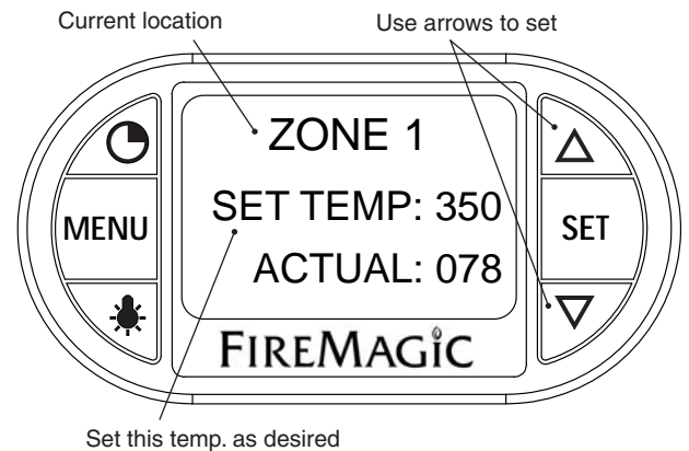
Fig. 26-1 Area temp. screen (zone 1 shown)
