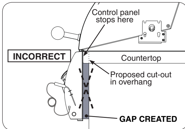
Fig. 18-1 Countertop overhang - incorrect cutout
