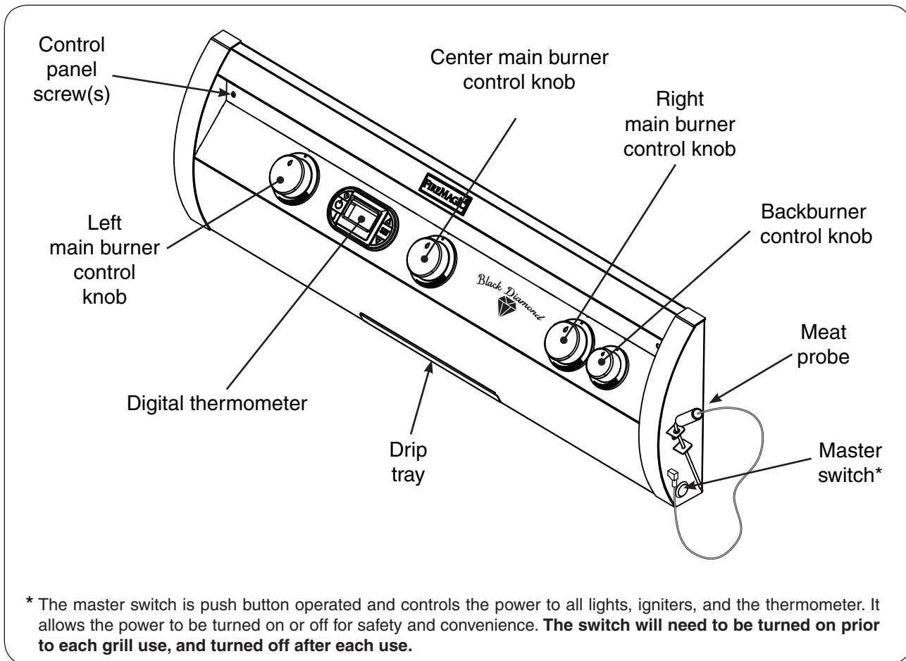
Fig. 22-1 H790i controls
