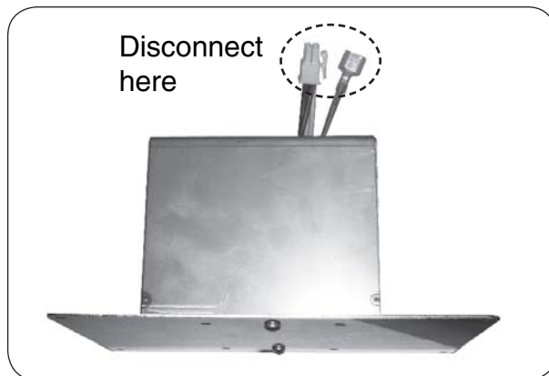
Fig. 35-2 Disconnect wire harness and groundwire (and power cord)
