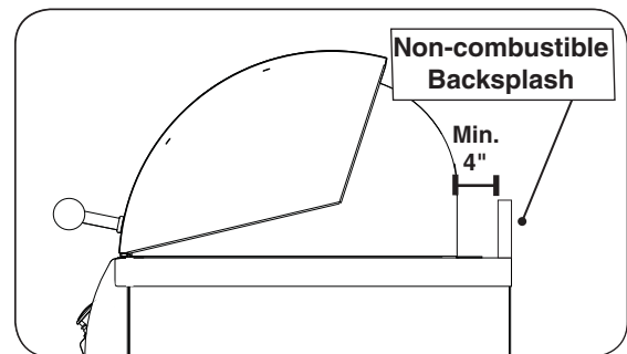
Fig. 12-5 Backsplash clearance
