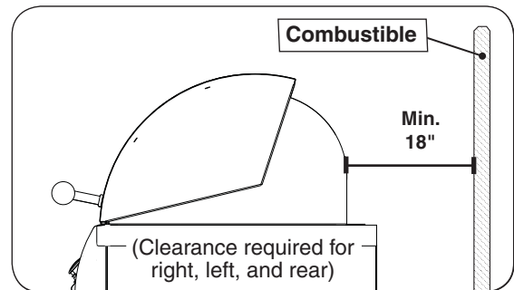
Fig. 12-4 Clearance 'C' Diagram
