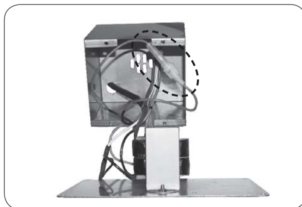
Fig. 35-4 Carefully open box and replace fuse (red wire)
