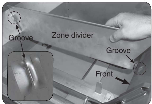
Fig. 19-2 Install zone dividers
