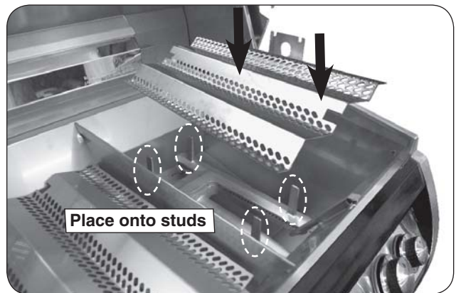
Fig. 19-3 Install flavor grids
