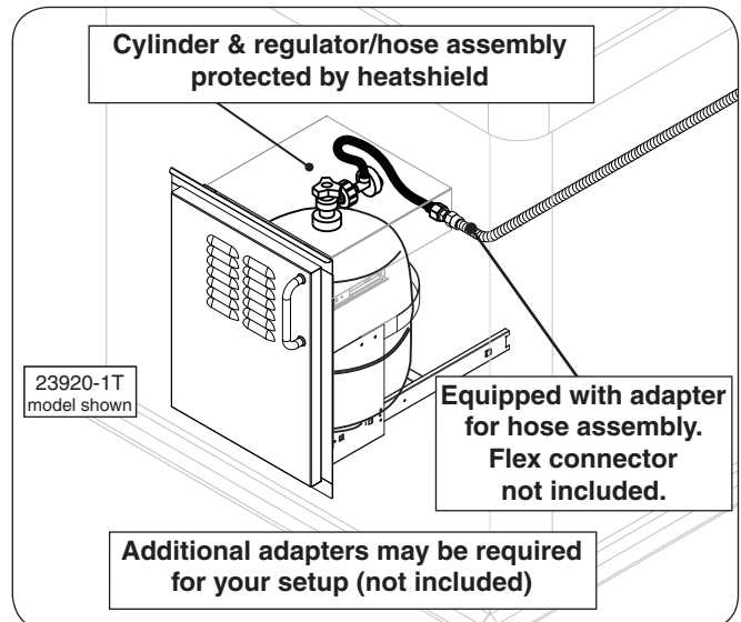
Fig. 14-3 Optional RHP door w/ tank tray
