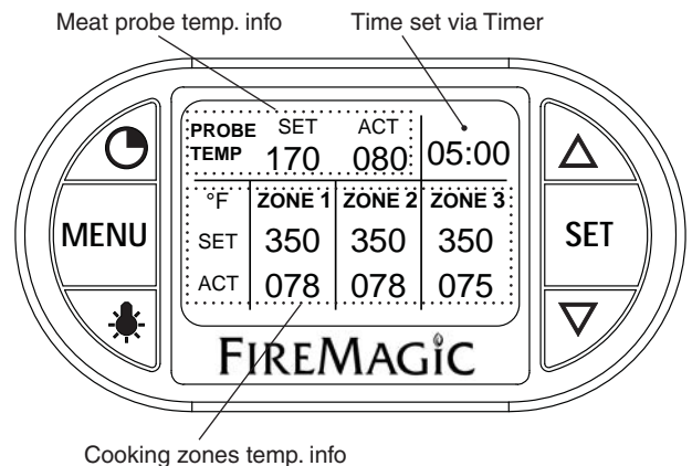
Fig. 25-3 Default screen detail
