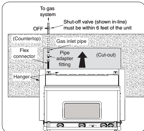
Fig. 18-4 Household propane & natural gas diagram
