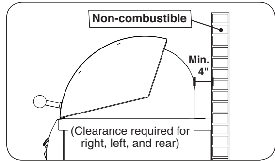
Fig. 12-2 Clearance 'A' Diagram
