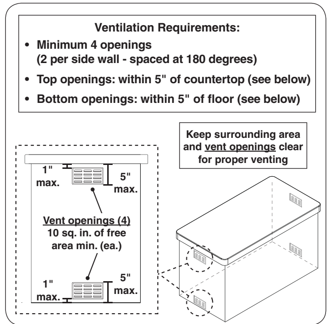
Fig. 14-1 Ventilation detail
