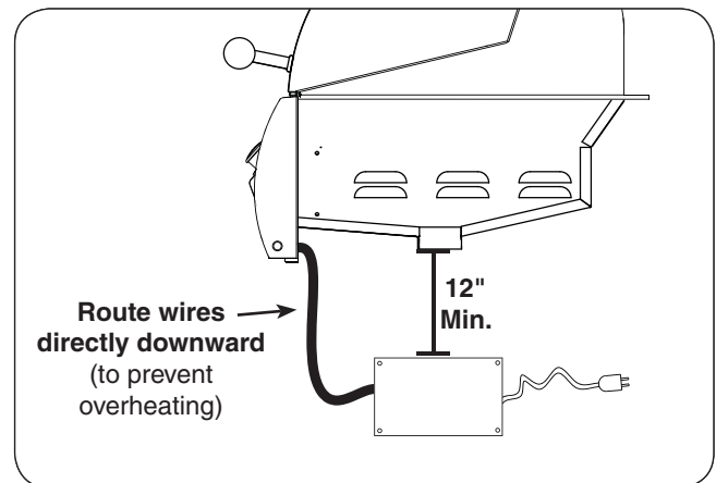
Fig. 21-3 Power supply clearance
