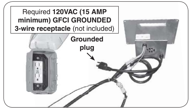
Fig. 21-1 Power supply detail
