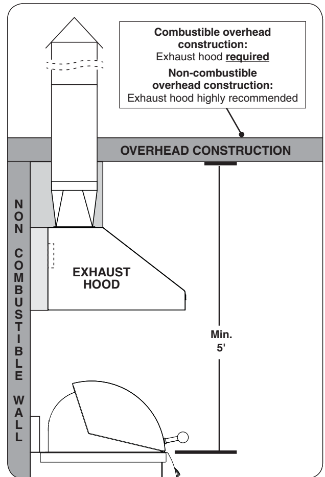
Fig. 11-1 Overhead requirements
