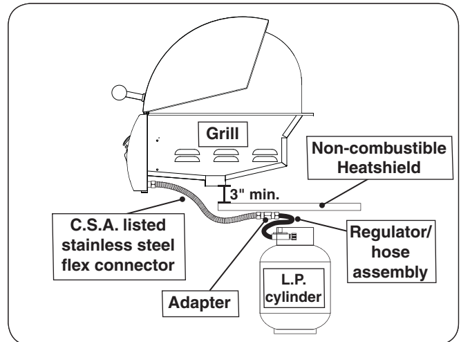
Fig. 14-2 Propane cylinder orientation
