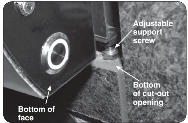
Fig. 19-1 Adjust support screws
