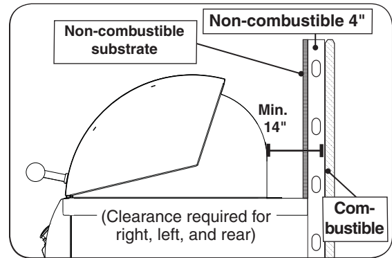
Fig. 12-3 Clearance 'B' Diagram
