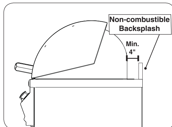
Fig. 9-4 Backsplash clearance
