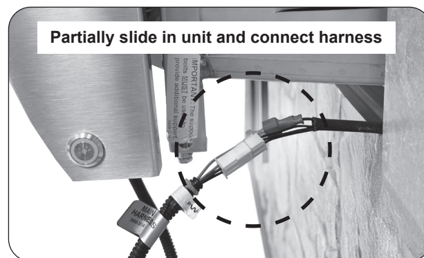
Fig. 26-3 Connect harnesses
