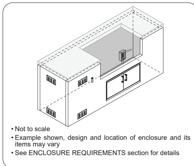
Fig. 26-1 Enclosure construction overview (if applicable)
