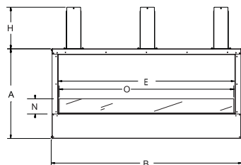
Single-Sided 48-inch Fireplace
