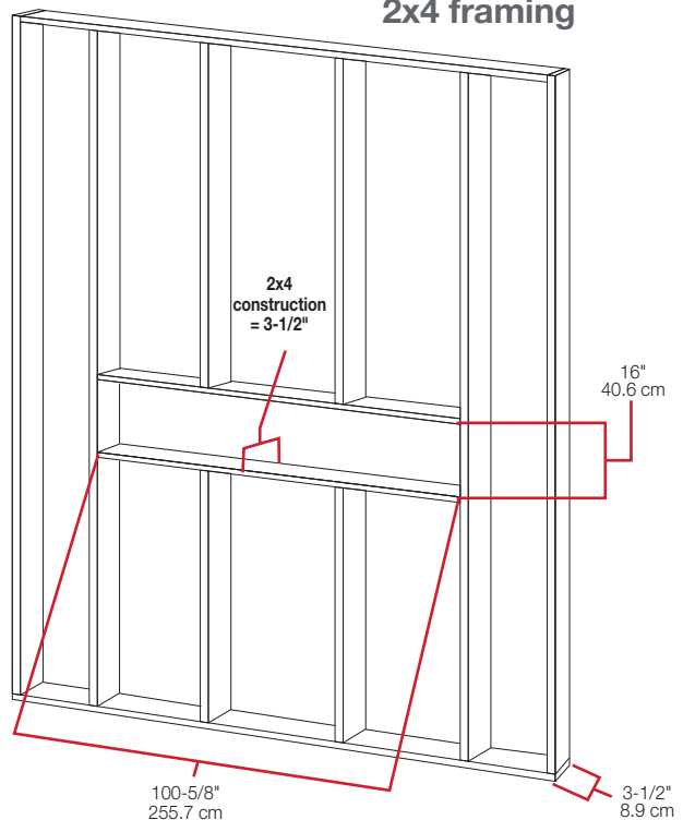
2x4 framing
