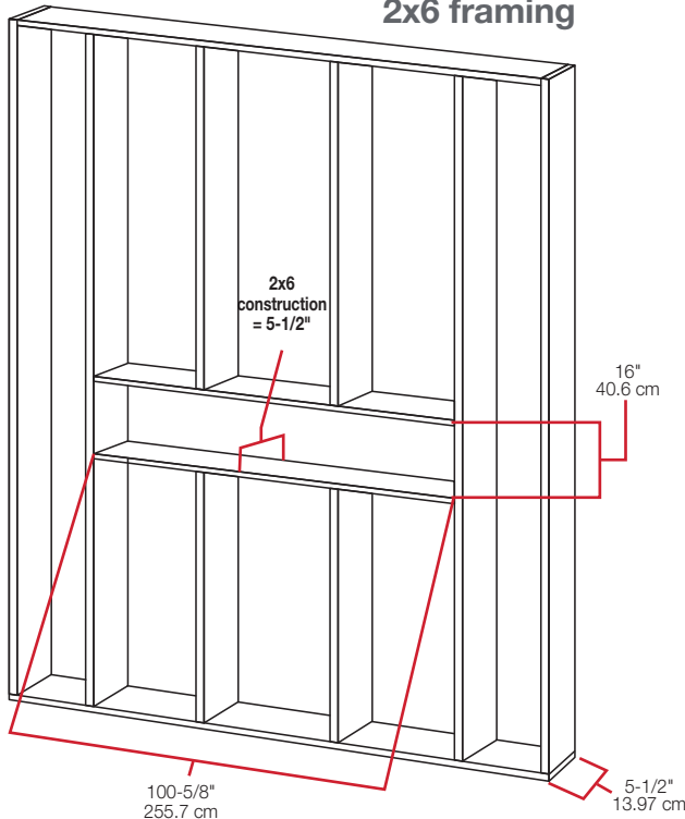
2x6 framing
