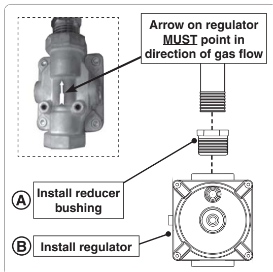
Fig. 2-2 Install bushing and regulator
