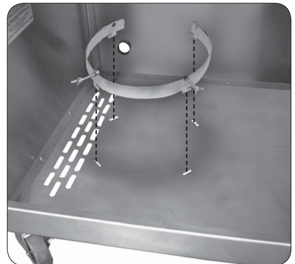
Fig. 5-3 Install tank ring
