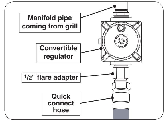
Fig. 5-1 Locate natural gas connections
