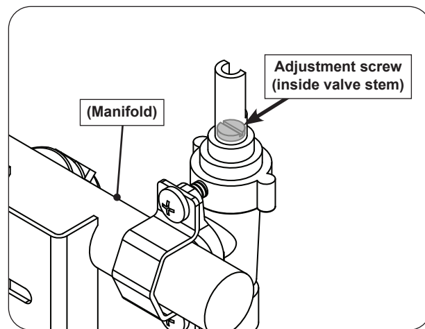
Fig. 33-1 Valve adjustment screw location
