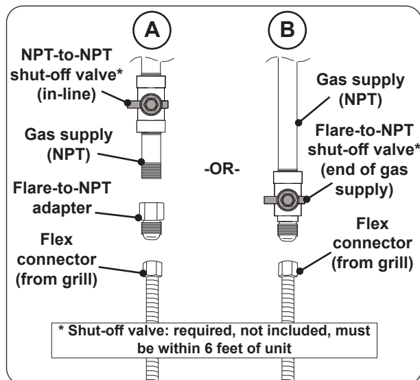
Fig. 30-1 Connecting to a gas line
