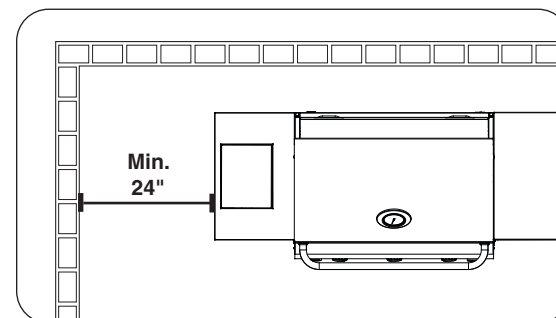
Fig. 9-4 Side/corner wall clearance
